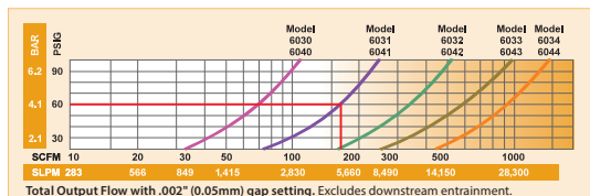
Metal parts are dried using a series of Model 6042 2" (51mm) Adjustable Air Amplifiers.
