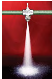
Model: AN1020SS Material: Type 303 Stainless Steel
